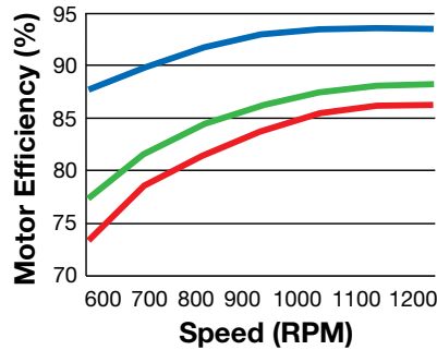
3HP Variable-Torque Application 1200 RPM Motor
