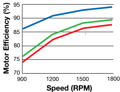
3HP Variable-Torque Application 1800 RPM Motor
