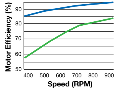
3HP Variable-Torque Application 900 RPM Motor
