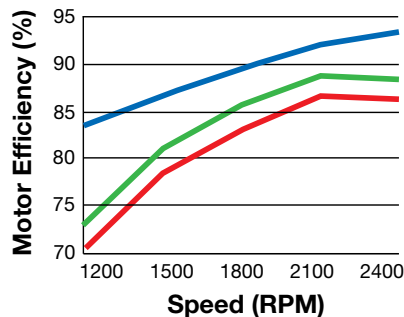
3HP Variable-Torque Application 2400 RPM Motor
