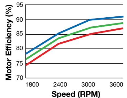
3HP Variable-Torque Application 3600 RPM Motor
