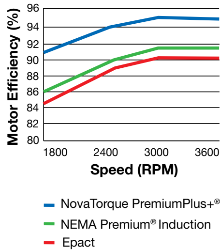
20HP Variable-Torque Application 3600 RPM Motor
