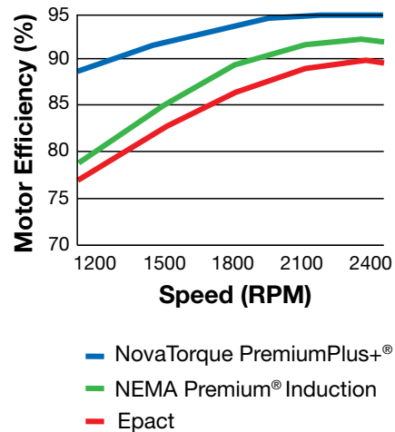
20HP Variable-Torque Application 2400 RPM Motor
