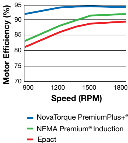
20HP Variable-Torque Application 1800 RPM Motor
