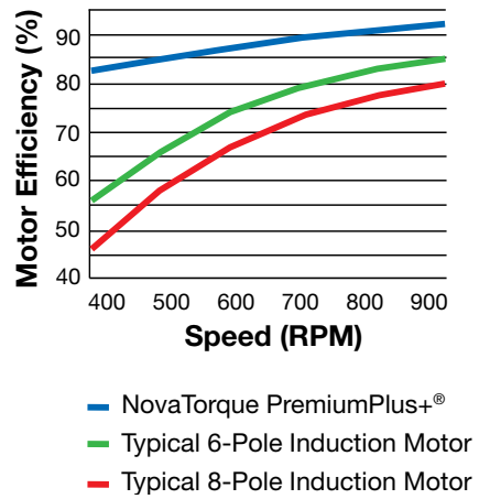
1HP Variable-Torque Application 900 RPM Motor
