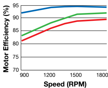
15HP Variable-Torque Application 1800 RPM Motor
