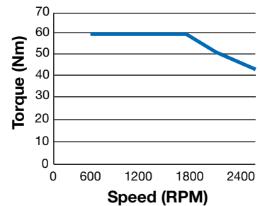
15HP Torque vs. Speed 1800 RPM Motor
