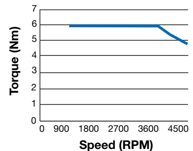
3HP Torque vs. Speed 3600 RPM Motor
