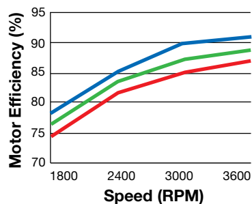
3HP Variable-Torque Application 3600 RPM Motor
