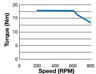
1.5HP Torque vs. Speed 600 RPM Motor
