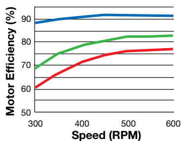
1.5HP Variable-Torque Application 600 RPM Motor
