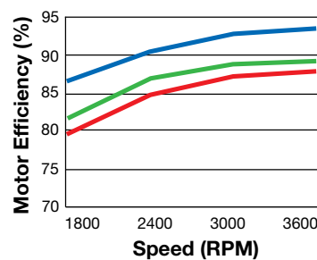
7.5HP Variable-Torque Application 3600 RPM Motor
