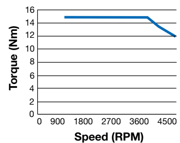
7.5HP Torque vs. Speed 3600 RPM Motor
