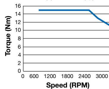
5HP Torque vs. Speed 2400 RPM Motor
