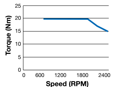
5HP Torque vs. Speed 1800 RPM Motor
