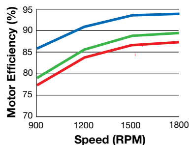
5HP Variable-Torque Application 1800 RPM Motor
